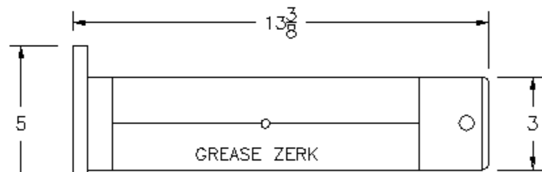
(2) LIFT CYLINDER HSG. TO LOWER PLOW ARM PART #4752-0026
