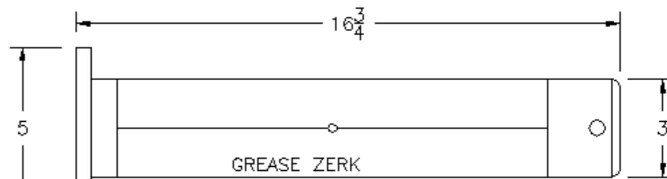
(2) REAR SWIVEL HEAD TO UPPER PLOW ARM (2) REAR SWIVEL HEAD TO LOWER PLOW ARM PART #4752-0027
