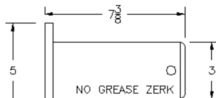
(2) PLOW BLADE TO SHAKER BOX BLADE MOUNT PART #4752-0028
