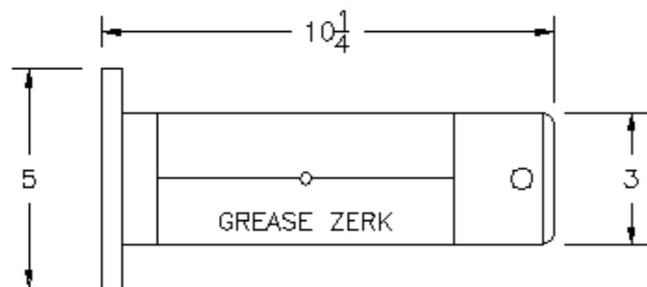
(2) LIFT CYLINDER HSG TO BACKPLATE PIVOT (2) REAR SWIVEL HEAD TO SHAKER BOX PIVOT PART #4752-0032
