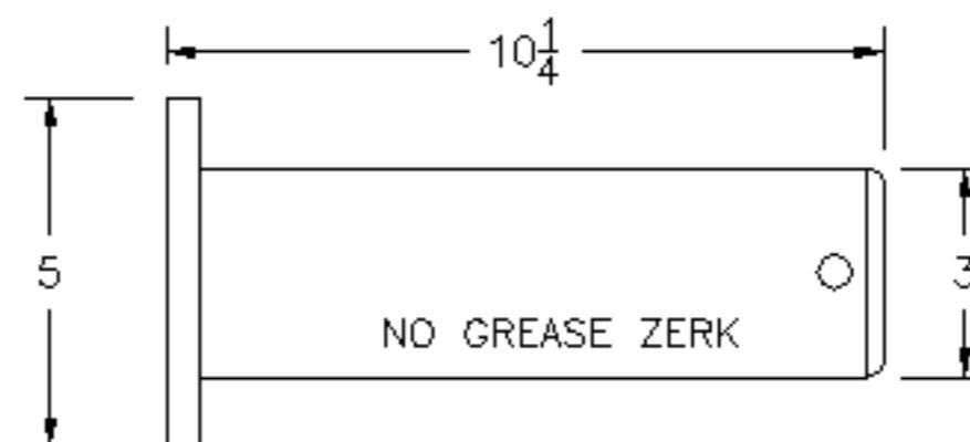
(2) STEERING CYLINDER T-END (2) SWING CYLINDER T-END PART #4752-0030
