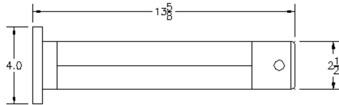
UPPER AND LOWER PLOW ARM PIN
