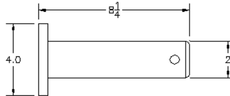
BACKPLATE T-END PIN
