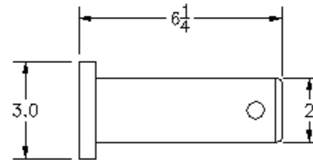
BLADE PIN
