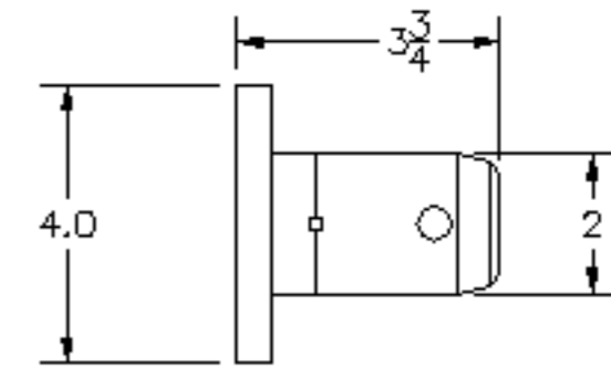
SINGLE REEL RACK PIVOT PIN
