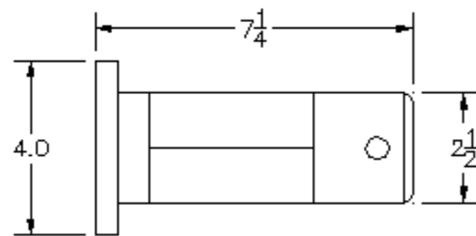
SWIVEL PIN
